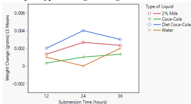
Figure 3.2: Interaction Plot between submersion time and liquid type on weight change
